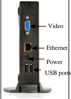
Connecting the RBT-070
